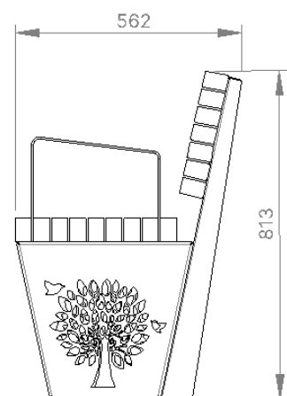
RIGHT
