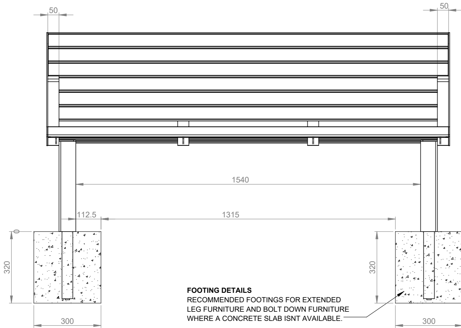
FRONT VIEW
