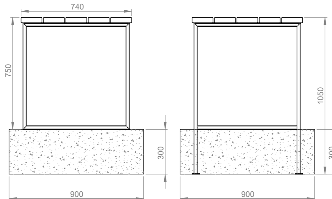
END VIEW (BOLT DOWN)
