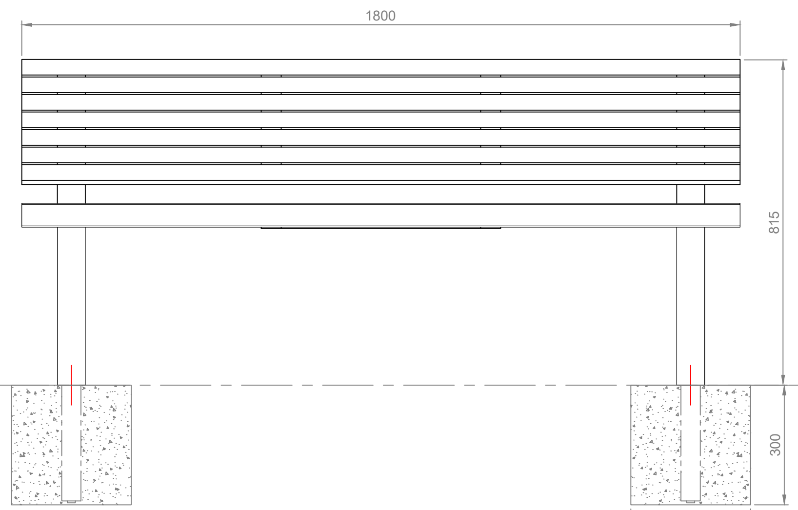
Front view
