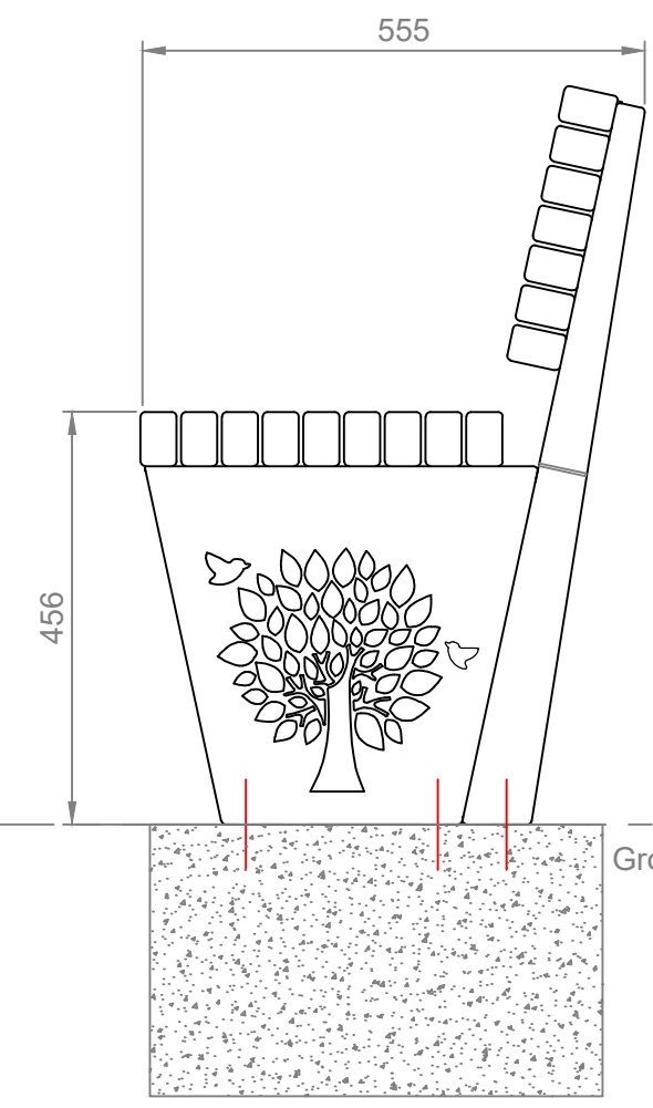
Right view
