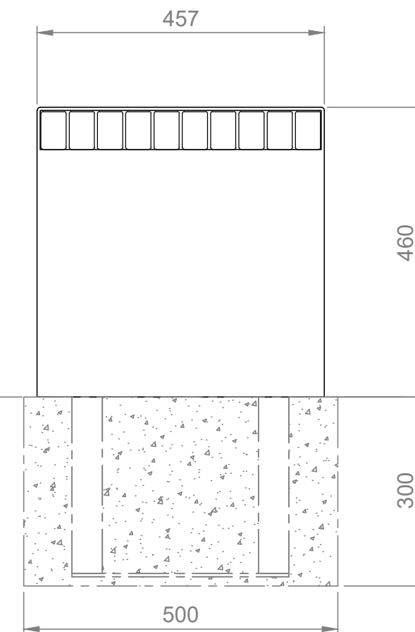
End View
