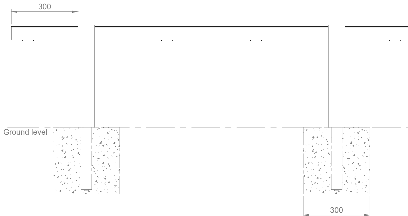
Front View
