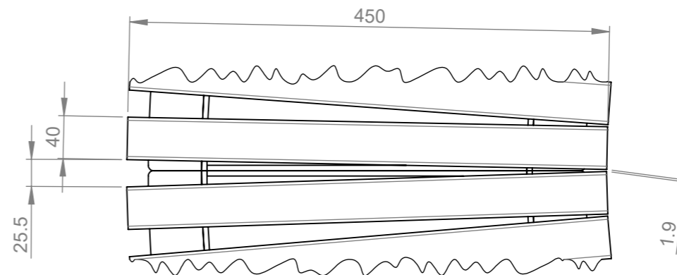
DETAIL A SCALE 1 : 5
