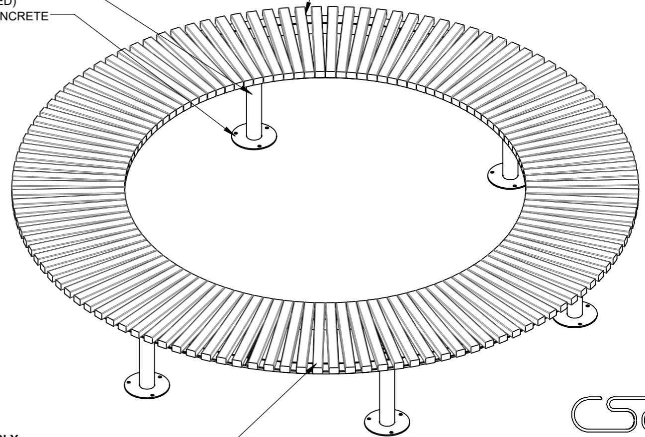
ISOMETRIC VIEW
