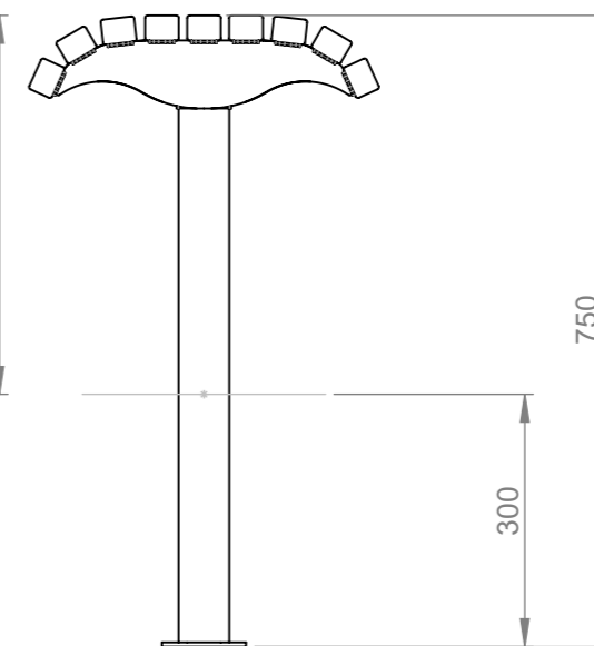
END VIEW (EXTENDED LEG)
