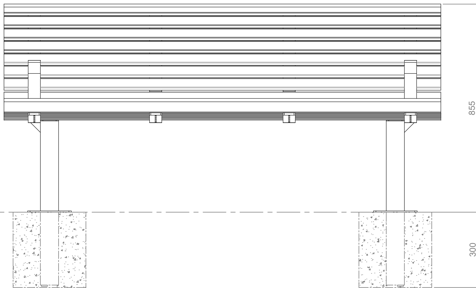
Front view
