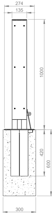
FRONT VIEW (REMOVABLE IN-GROUND SLEEVE)
