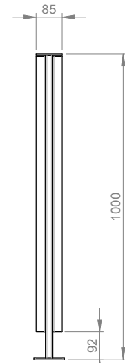
RIGHT VIEW (BASE PLATED)
