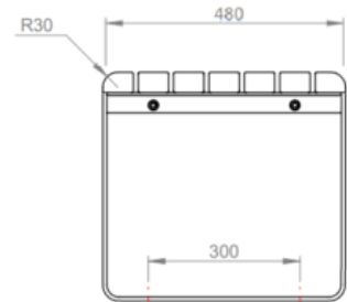
RIGHT VIEW
