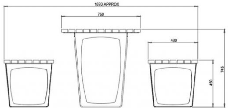
END VIEW
