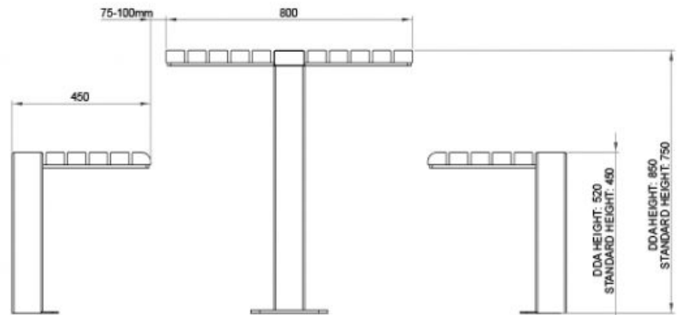
END VIEW
