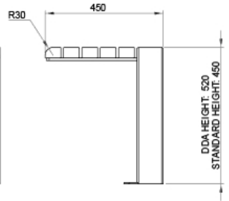
END VIEW
